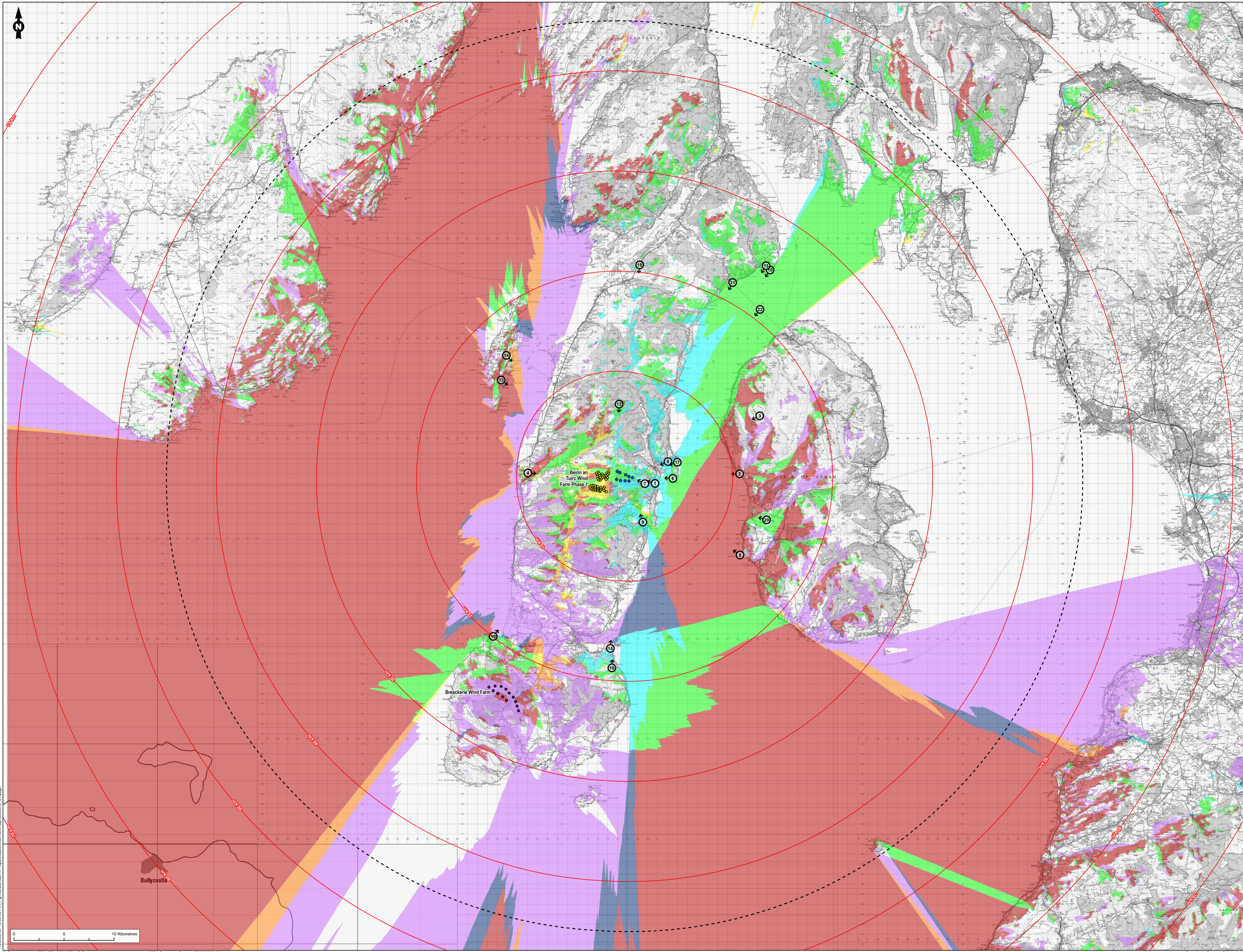
Figure Title Cumulative ZTV: Proposed Development, Beinn an Tuirc Wind Farm Phase 1 and Breackerie Wind Farm
