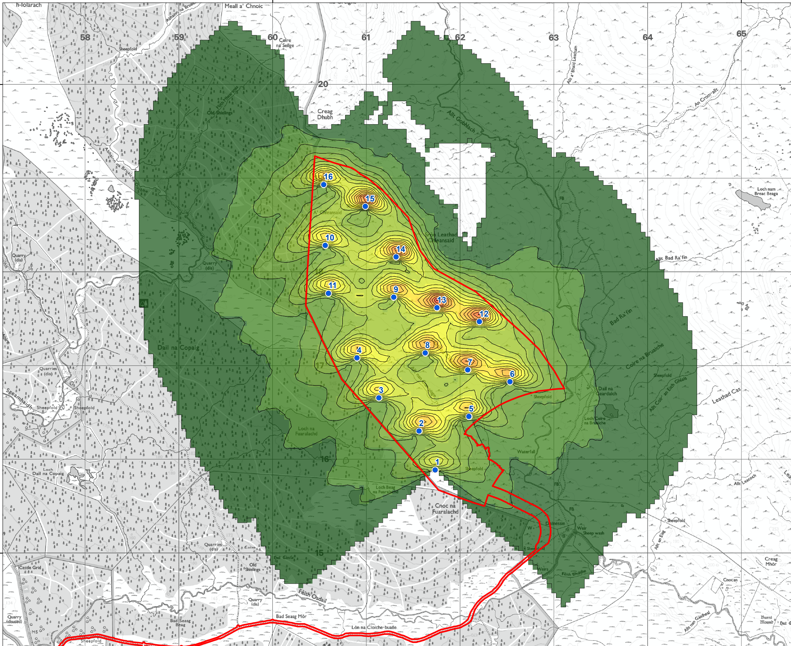
TITLE: Figure 15.1: Shadow Flicker Area Worst Case Scenario
