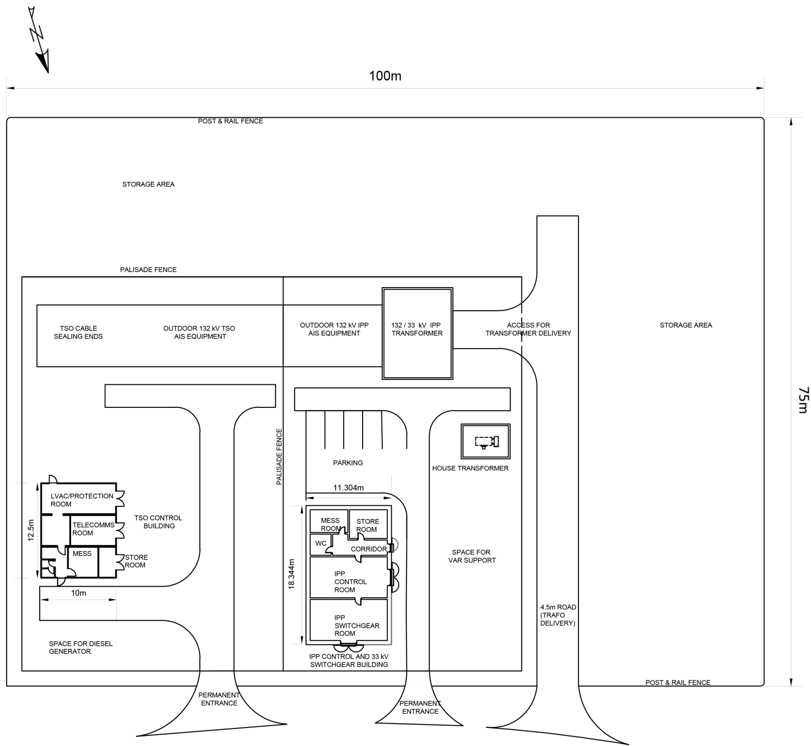
SUBSTATION PLAN SCALE 1:500
