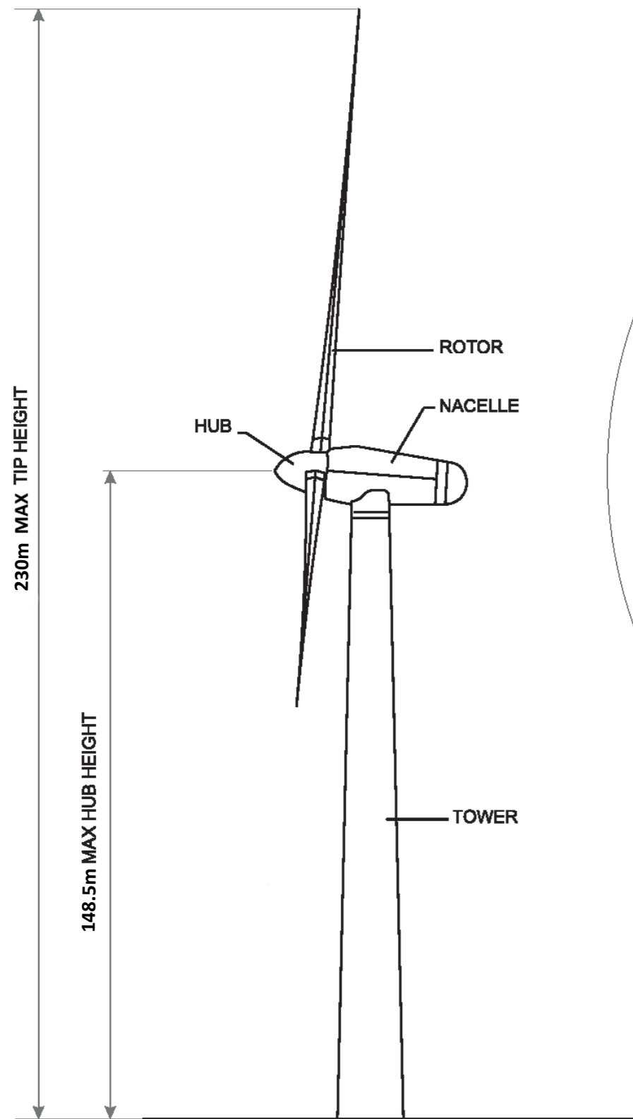
SIDE ELEVATION
