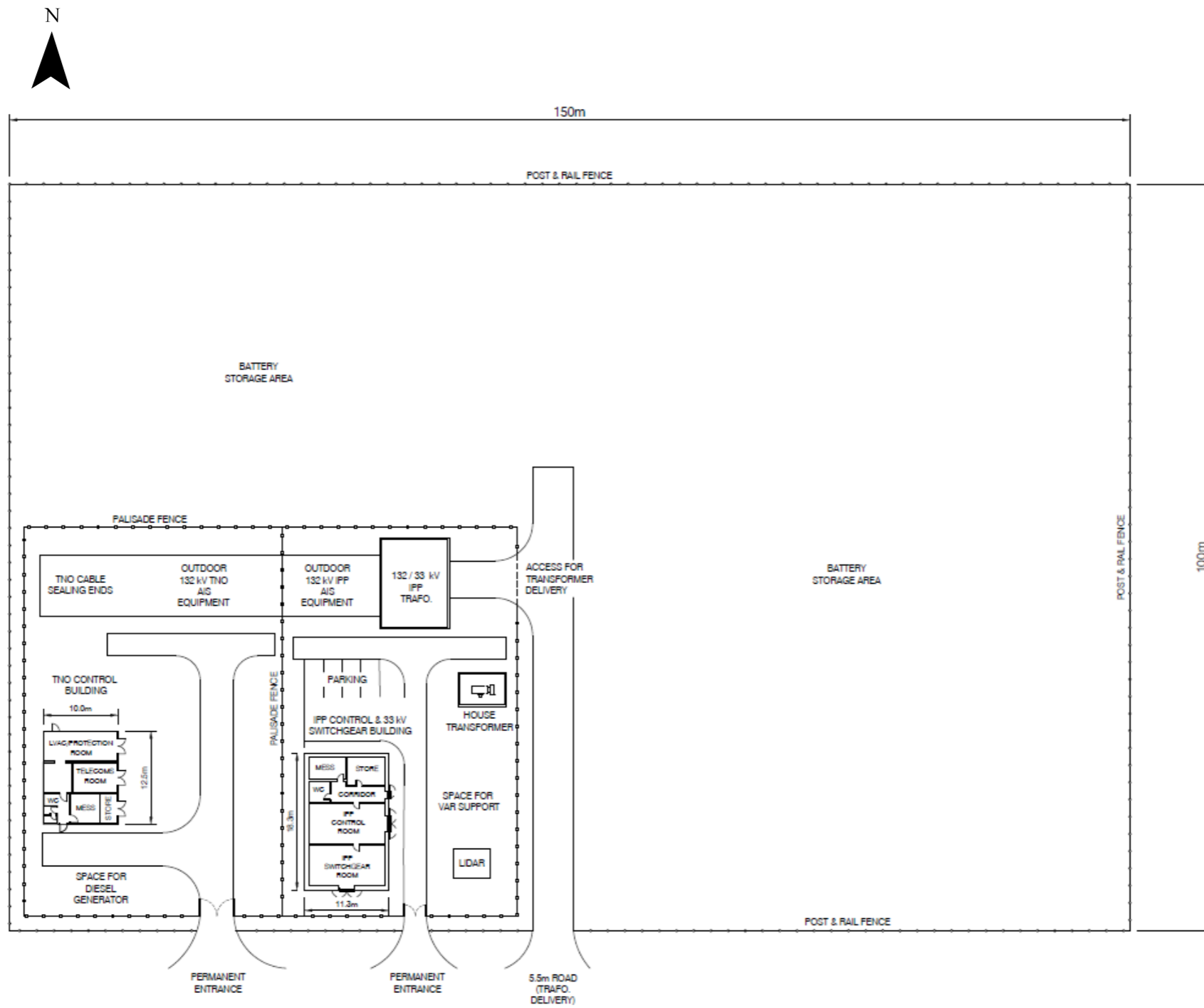
SUBSTATION COMPOUND PLAN SCALE 1:500
